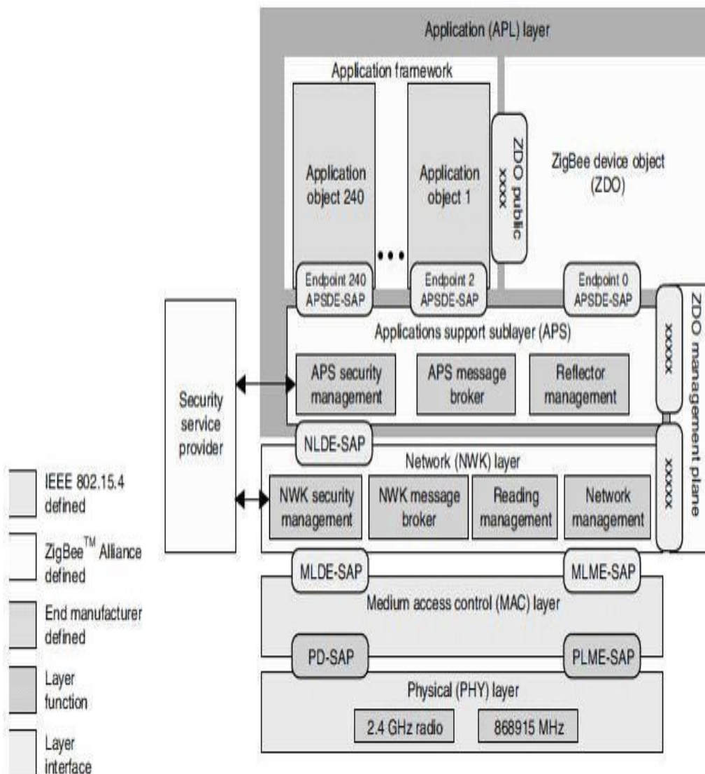
Fig. 3. A detailed overview of ZigBee stack Architecture
