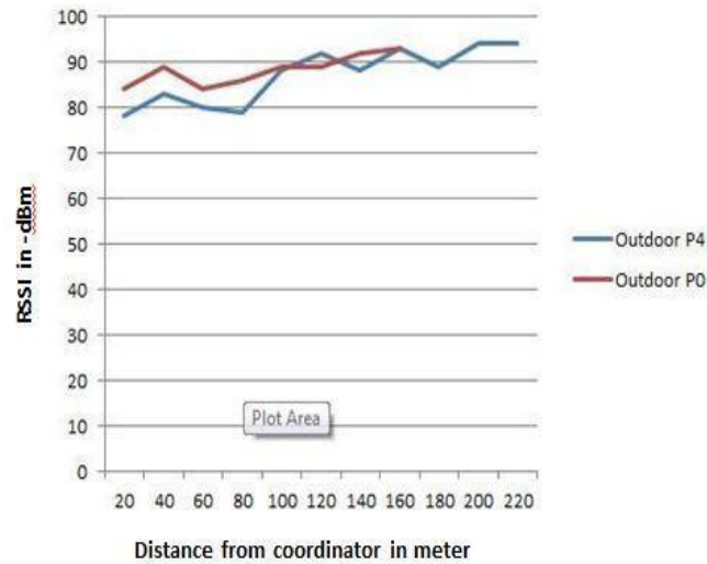
Fig 11: Measurement of RSSI value vs. distance at transmit power level P0 and P4.
