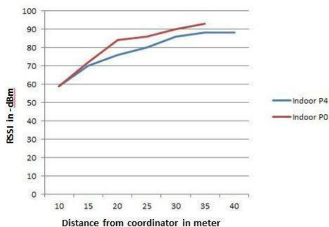
Fig 10: Measurement of RSSI value vs. distance at transmit power level P0 and P4.
