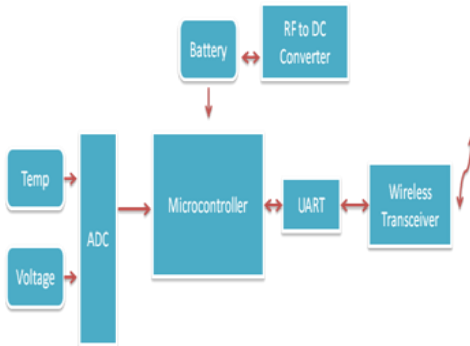
Fig 4:Block Diagram
