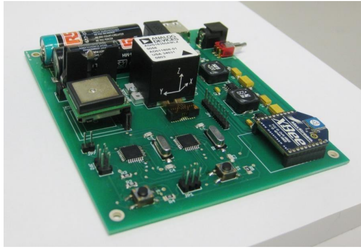
Fig. 2 Picture of the system prototype
