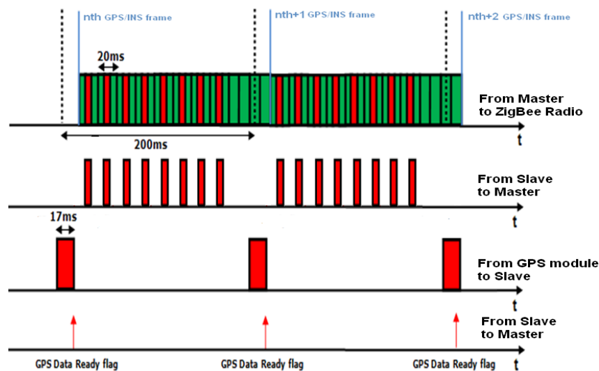
Fig. 4 GPS/Inertial data timing (in red the GPS data, in green the inertial data)
