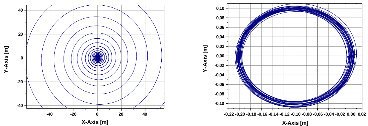
Fig. 15 Trajectory reconstruction without (left) and with (right) Kalman filtering
