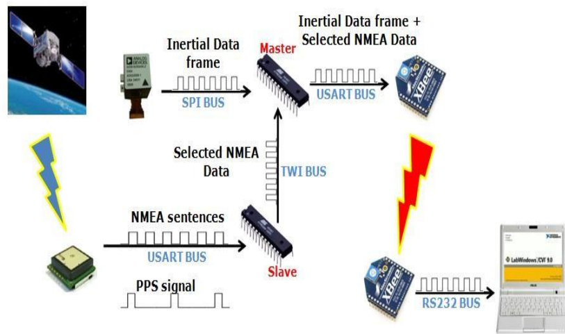
Fig. 3 System operations
