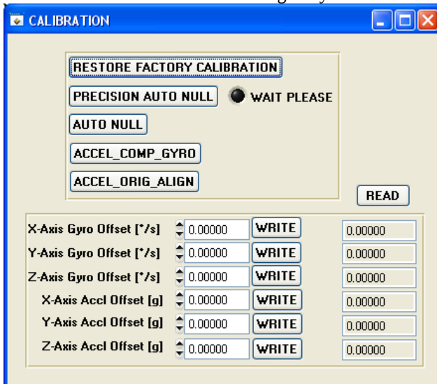
Fig. 8 Calibration sub-window
