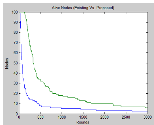
Fig. 5 Comparative Analysis (Existing Vs. Proposed) Alive Nodes
