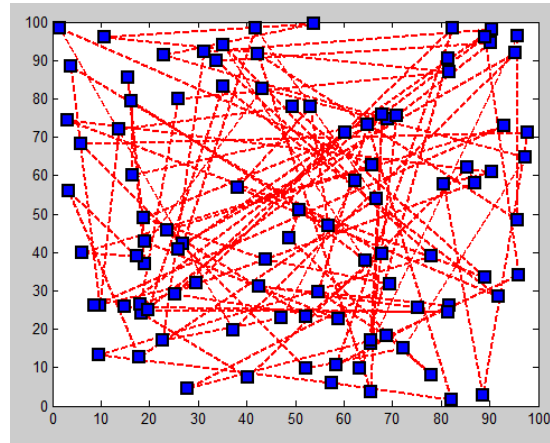
Fig.2 The chain formed in exiting pegasis Protocol
