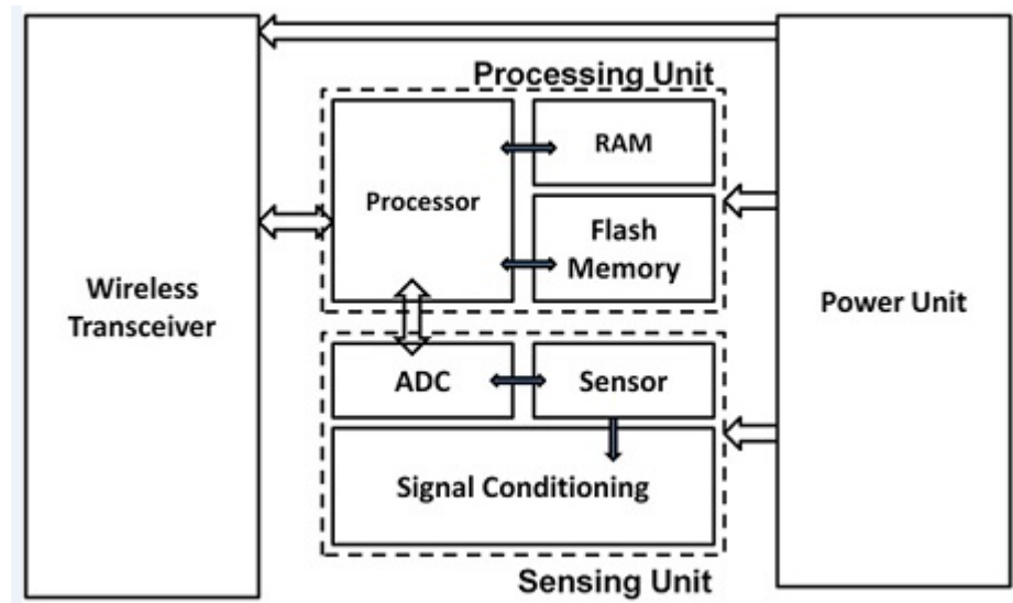
Fig. 1 Schematic of a Wireless Sensor Network Architecture
