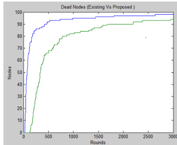
Fig. 4 Comparative Analysis (Existing Vs. Proposed) Dead Nodes
