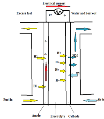
Figure 4 PEM fuel cell [14]
