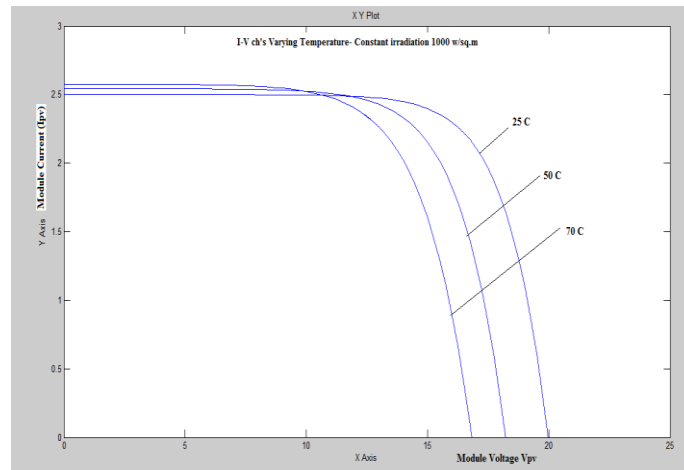
Figure 9 current -voltage graph vary Temperature- Constant irradiation 1000 w/sq.m
