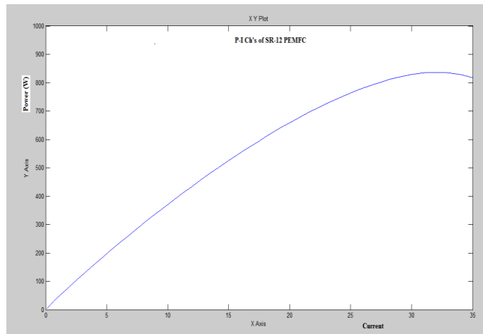
Figure 12 P-I characteristic of SR-12 module
