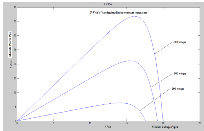
Figure 8 Power - Voltage graph - vary irradiation- Constant temperature 25°C
