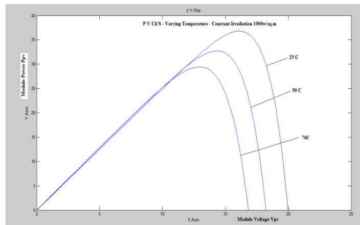
Figure 10 Power - Voltage graph Vary Temperature- Constant irradiation 1000 w/sq.m
