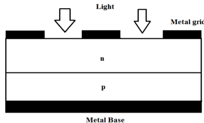
Figure 1 Construction of Photovoltaic cell [13]
