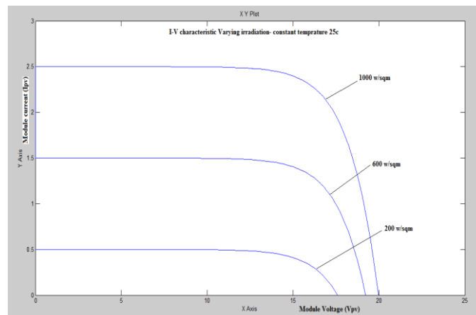
Figure 7 current - voltage graph - vary irradiation- Constant temperature 25°C
