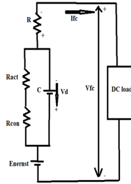
Figure 6 Electrical identical circuit of the PEM fuel cell [7]
