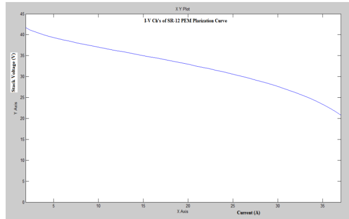
Figure 11 characteristic of SR-12 PEM polarization curve
