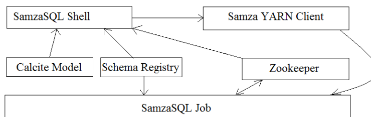
Fig. Streaming SQL Architecture
