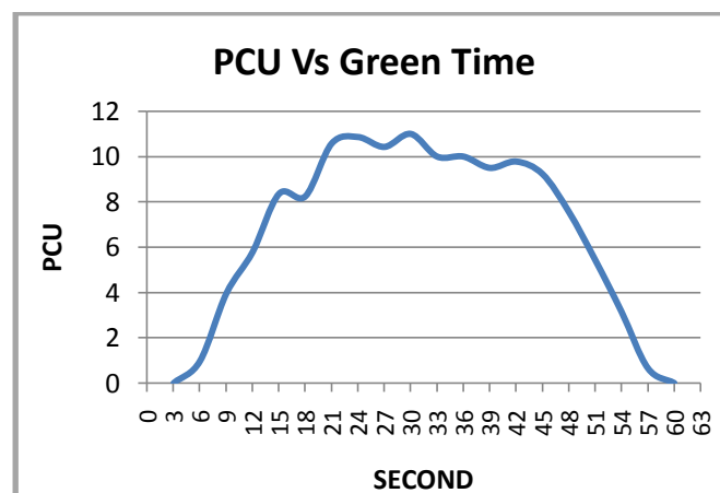
Fig.:7 Highly saturated cycle of phase 2 of intersection at morning peak hour
