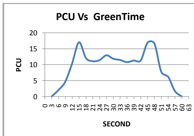
Fig.: 4 Highly saturated cycle of phase 1 of intersection at evening peak hour
