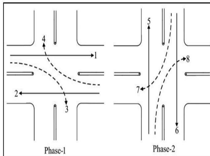
Fig.: 8 Two Phase Signal
