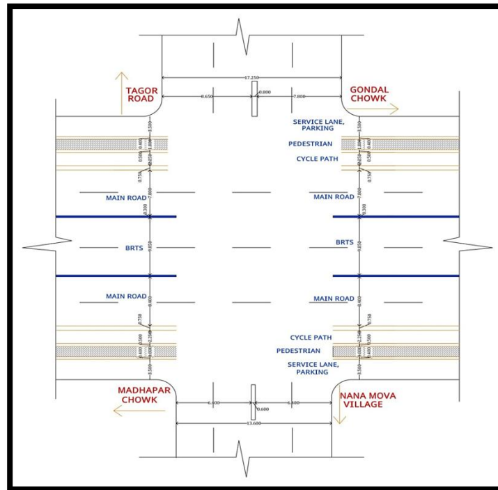
Fig.: 1 Road Inventory Features of Nana Mauva Intersection
