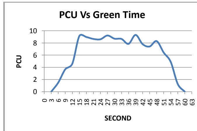
Fig.:6 Highly saturated cycle of phase 1 of intersection at morning peak hour
