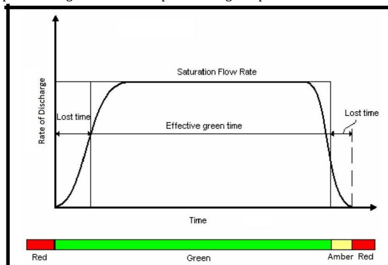
Fig.: 3The flow of traffic during the green period from a saturated approach
