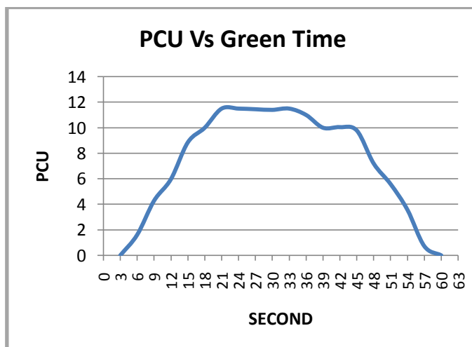
Fig.:5 Highly saturated cycle of phase 2 of intersection at evening peak hour
