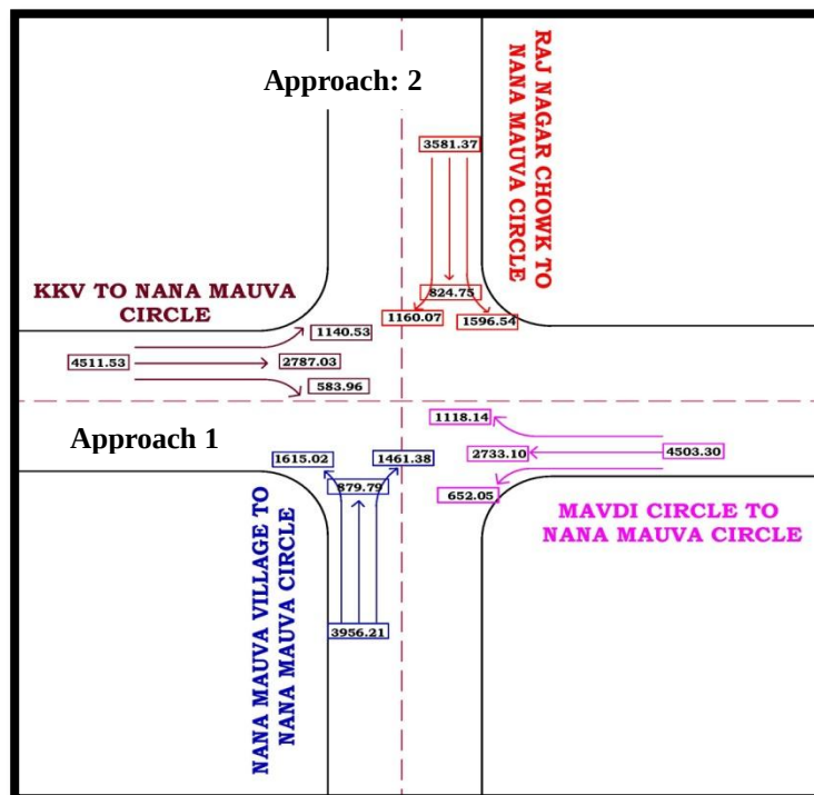
Fig.: 2 Demand Flow PCU/Hr at Intersection
