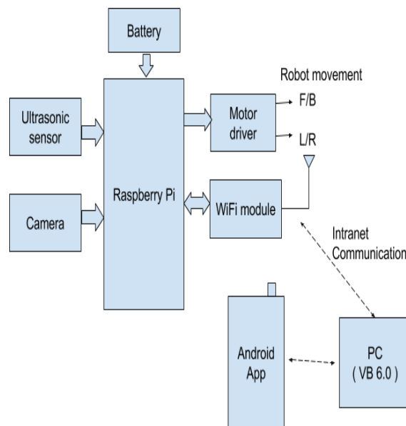
Fig.1 setup
