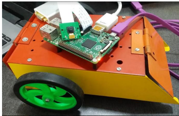
Fig.1 setup
