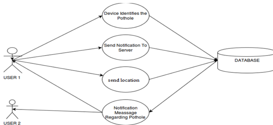
Fig4.UML diagram
