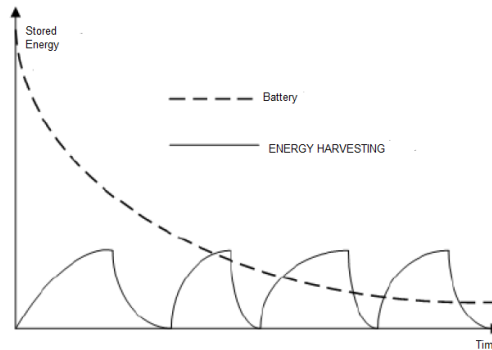
Fig.2.EH-WSN versus battery-operated WSN
