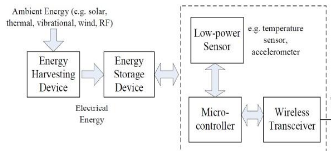
Fig.3. EH-WSN node energy module
