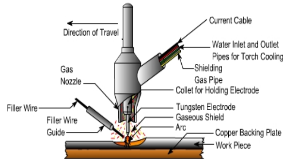
Figure 3 Gas tungsten arc welding
