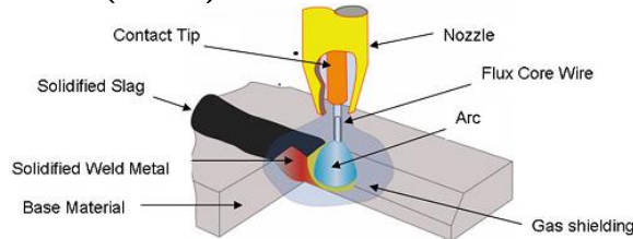
Figure 4 Flux cored arc welding
