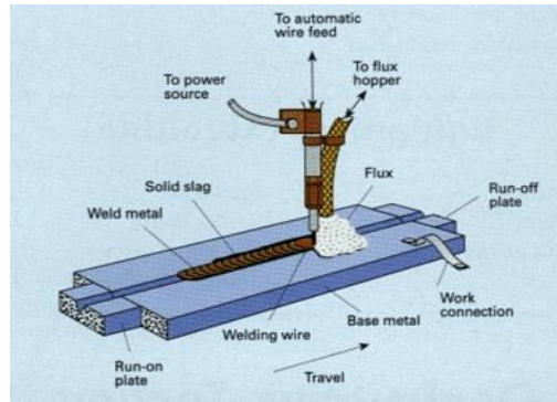
Figure 2 Submerged arc welding
