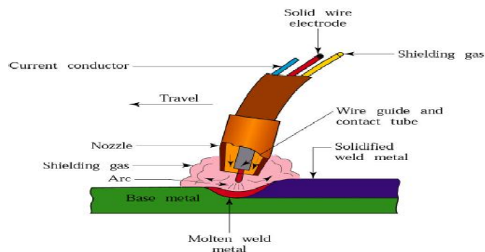
Figure 1 Gas metal arc welding
