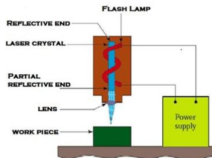
Figure 6 Laser beam welding
