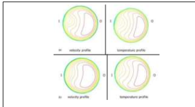
Fig. 10. Velocity and Temperature profiles at the exit of the tube for (a), constant properties and (b), temperature dependent properties [1]
