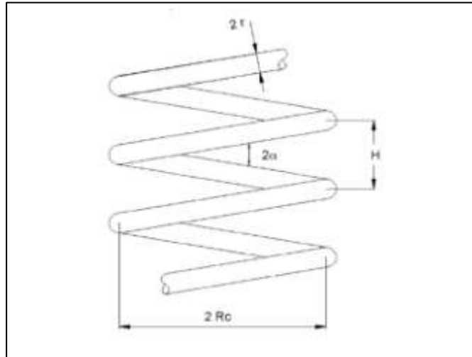
Fig. 1. Nomenclature of Helical Coil Heat Exchanger [1]
