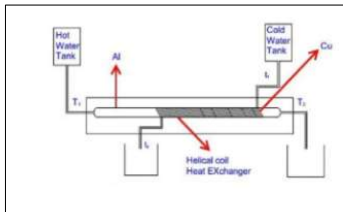
Fig. 6. Experimental setup[2]
