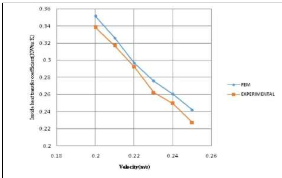
Fig. 16. Variation of Heat transfer coefficient vs. Velocity for experimentation and FEM results[3]
