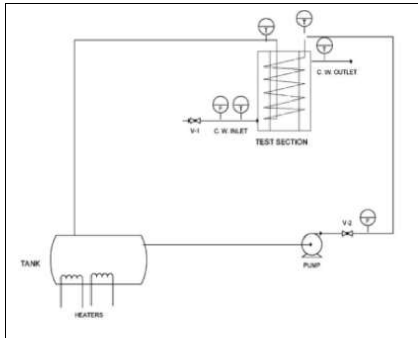
Fig. 4. Block diagram of Experimental Setup[1]
