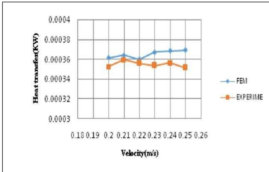
Fig. 15. Variation of Heat transfer vs. Velocity for experimentation and FEM results[3]
