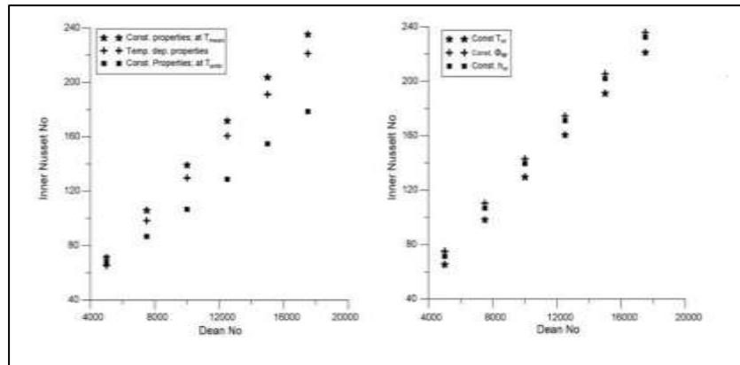
Fig. 5. Variation of Inner Nusselt number vs. Dean number at various properties at the wall and mean values of Temperature heat flux and heat transfer coefficient[1]
