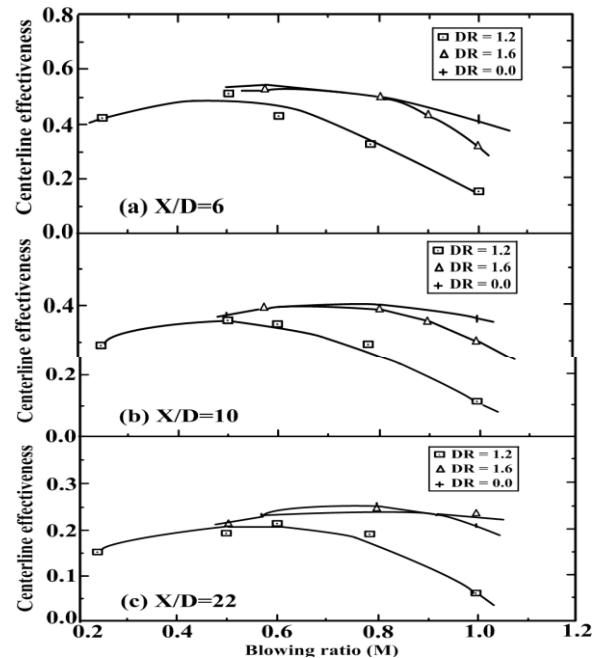
Fig.6 Effect of blowing ratio and density ratio on film effectiveness (a) X/D = 6 (b) X/D = 10 (c) X/D = 22
