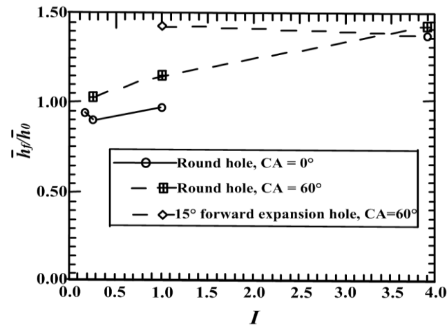
Fig.3 heat transfer coefficient ratios
