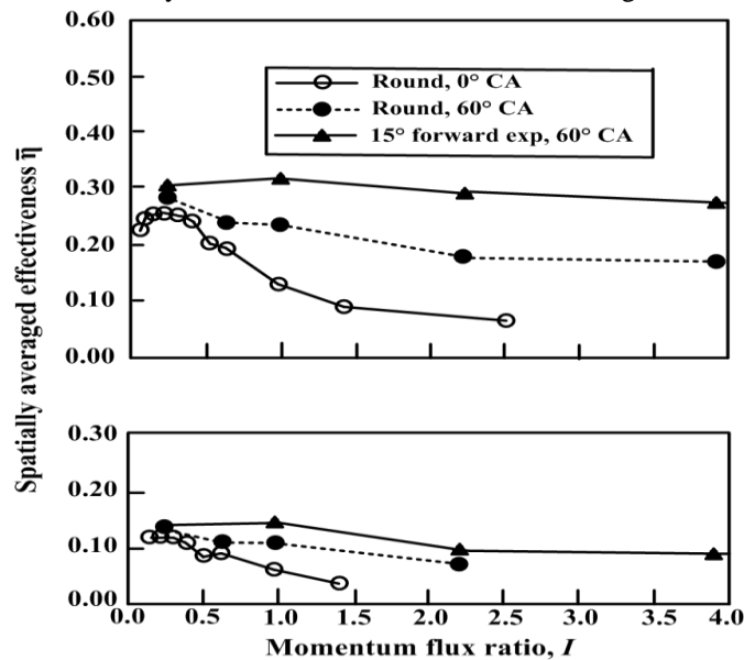
Fig.4 film cooling effectiveness for configurations
