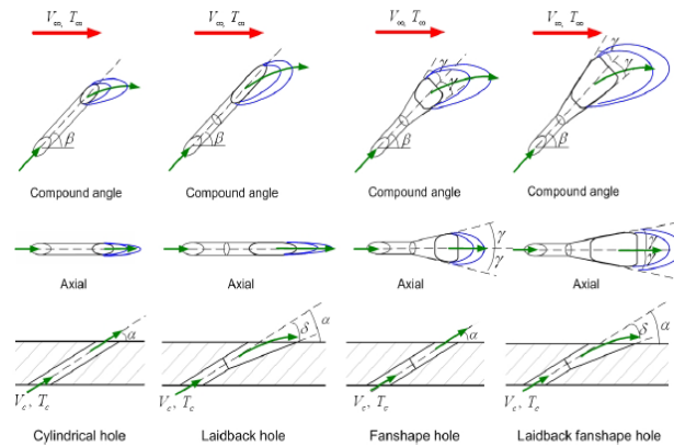
Fig.1 Film cooling hole configurations
