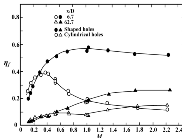
Fig.2 Comparing diffuser hole performance with cylindrical hole
