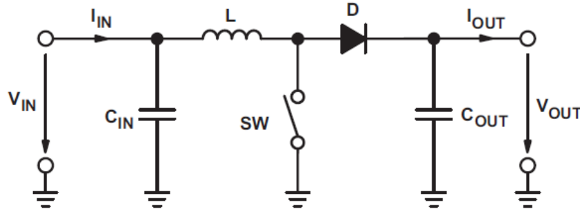
Figure 6: Boost Converter
