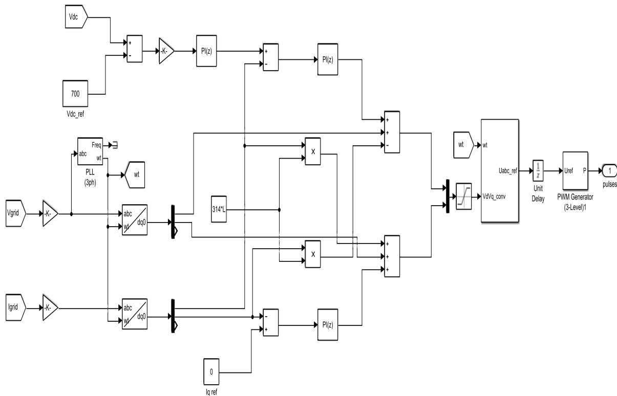
Figure 10: Feed forward control loop
