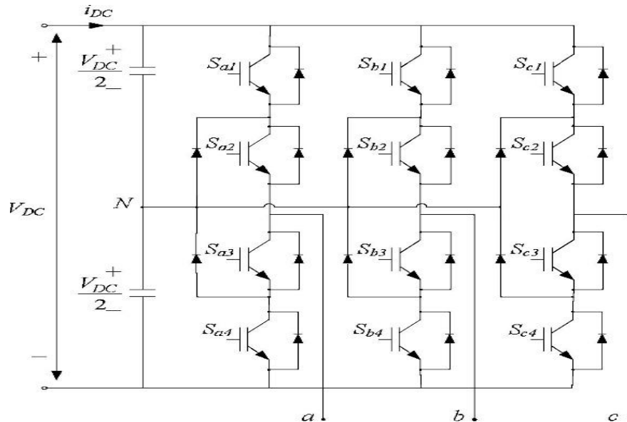
Figure 8: Three phase Three level NPC VSI [3]
