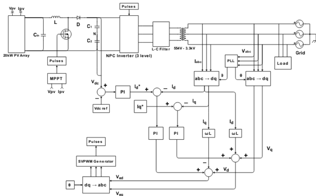
Figure 8: Control Block diagram of Grid tie PV System
