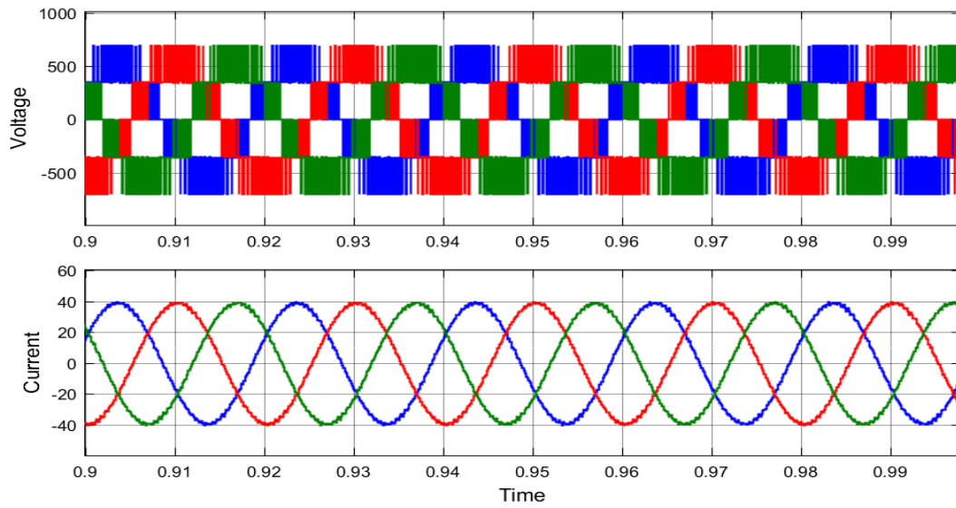
Figure 11: Three phase inverter voltage and current waveforms (before filter)
