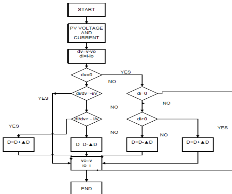
Figure 7: Incremental Conductance Algorithm
