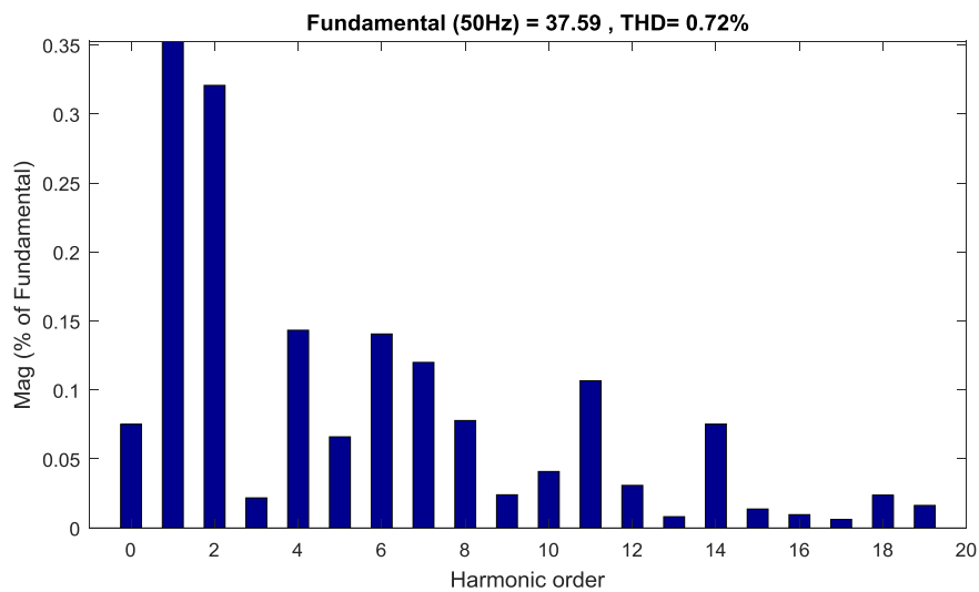
Figure 13: THD analysis of the current waveform at 2kHz switching frequency
