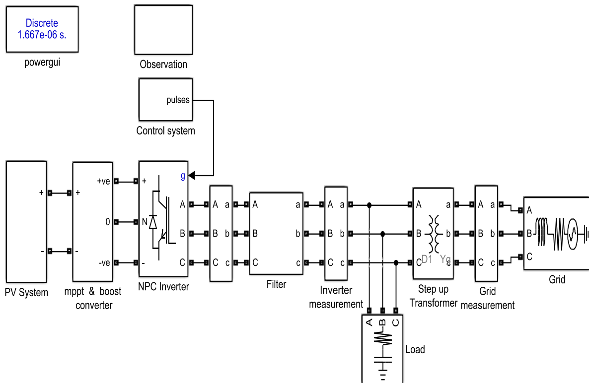
Figure 9: Grid tie PV array using Multilevel Inverter
