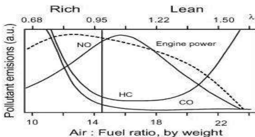
Fig. 1 Effect of A/F ratio on engine emissions and engine power
