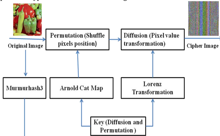
Figure 1. Architecture of the proposed encryption scheme
