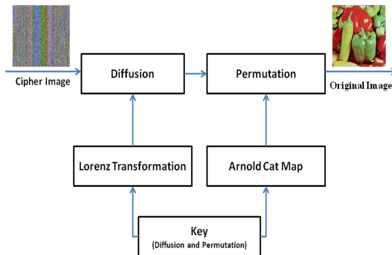
Figure 2. Architecture of the proposed decryption scheme
