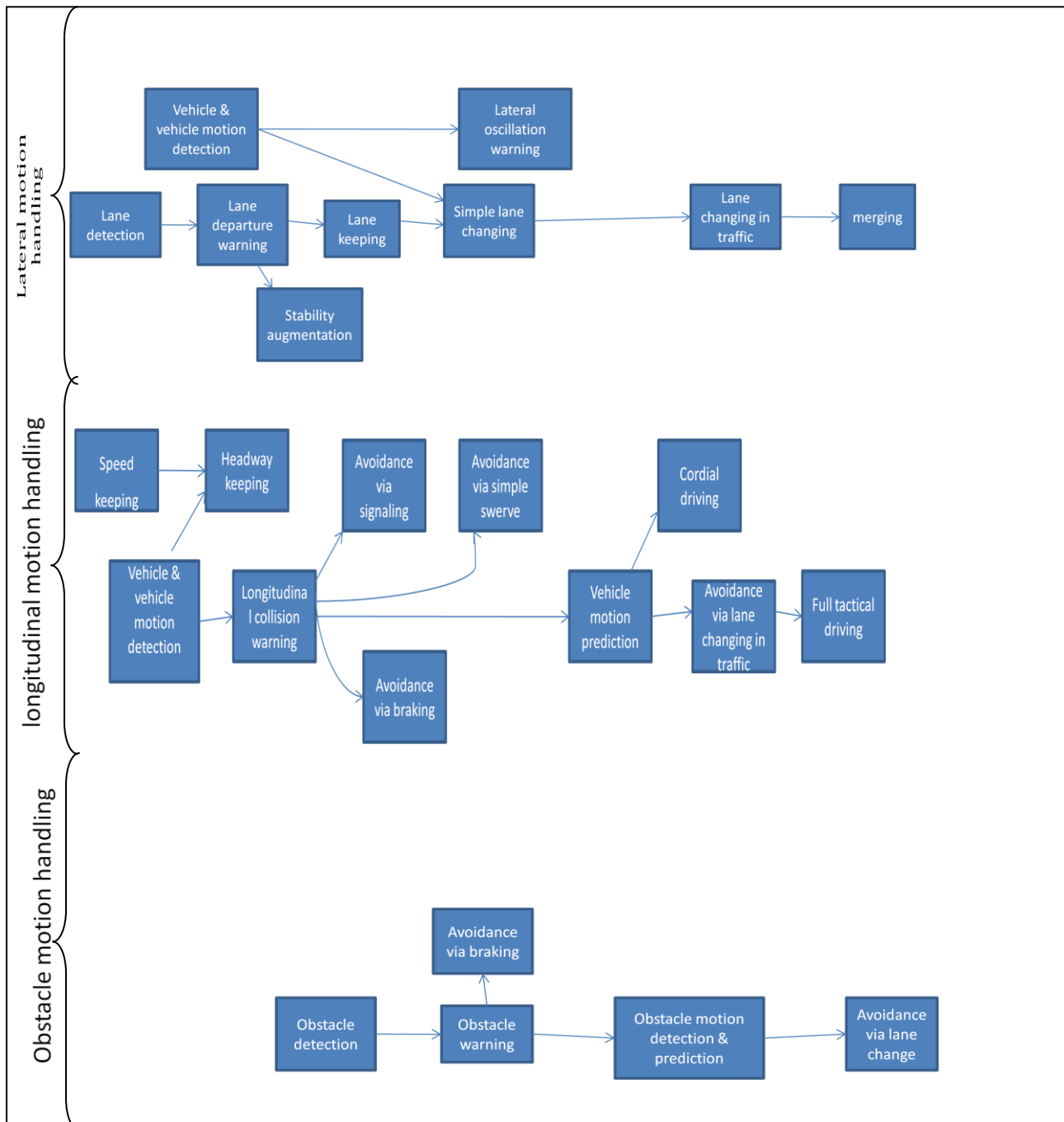
"Figure 3. Baseline Autonomous Reference Model"
