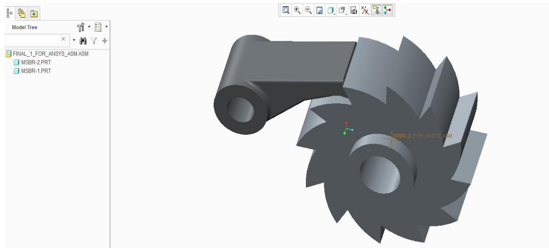
Figure 1: Ratchet-Pawl Assembly
