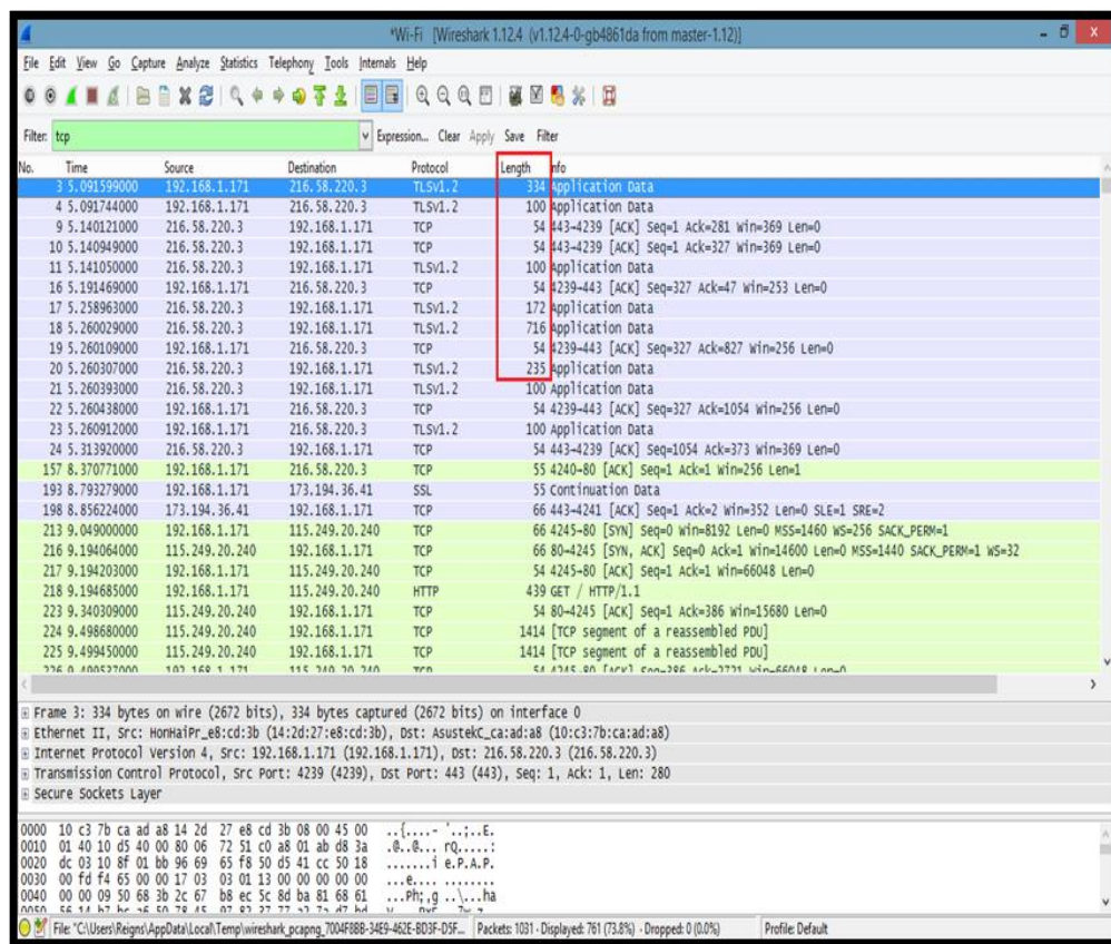
Figure 5. Packet Capture
