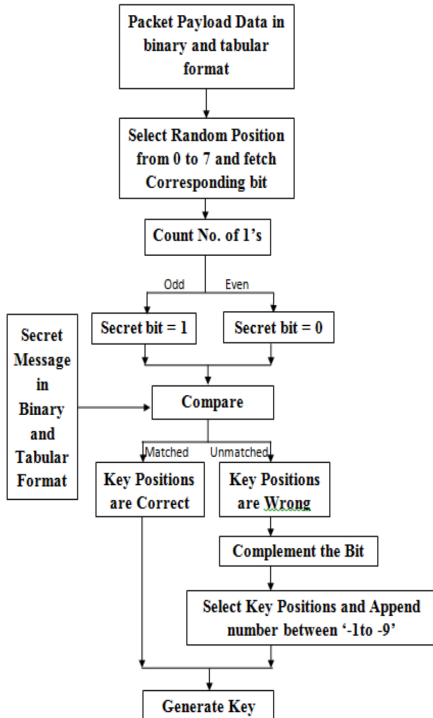
Figure 3. Key Generation
